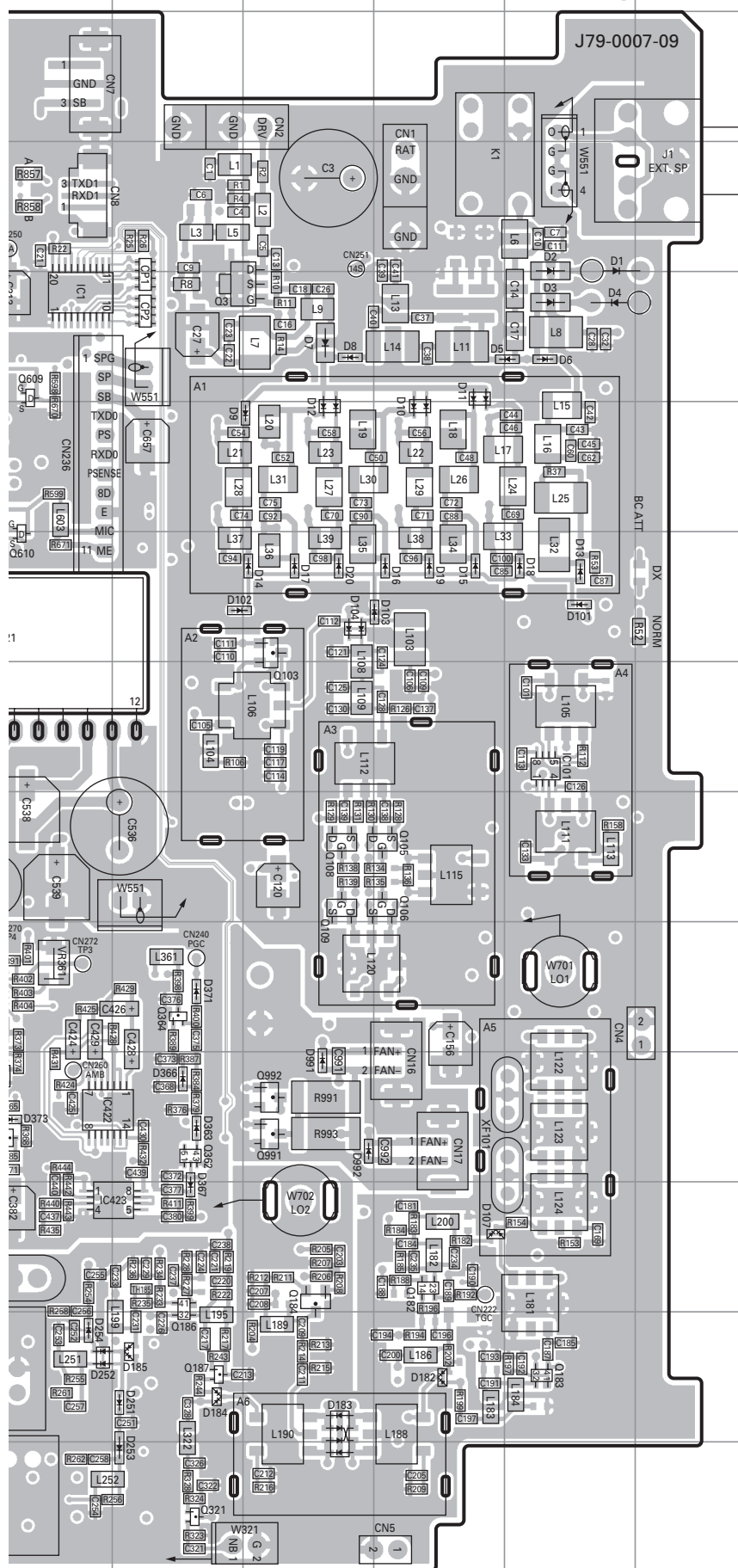
TX-RX UNIT (X57-7210-20) Component side view (J79-0007-09)
