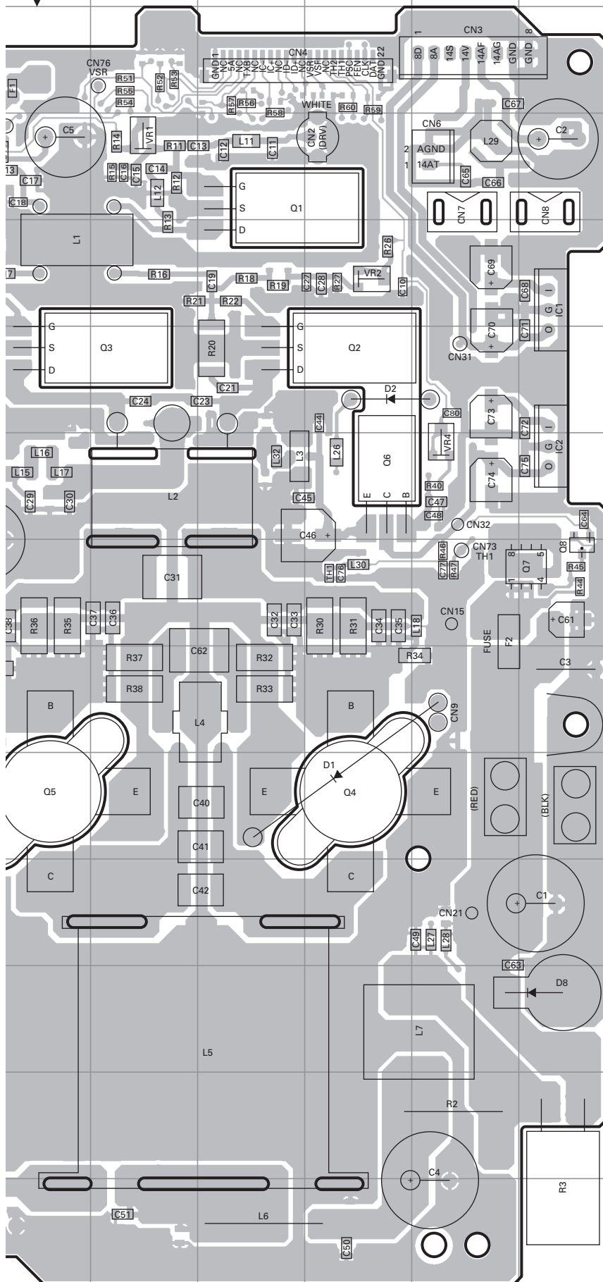
FINAL UNIT (X45-3780-20) Component side view (J79-0008-09)
