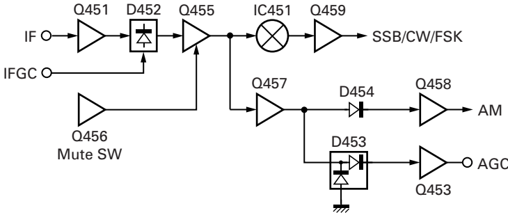
Fig. 5 From the receiving second IF amplifier to detection and AGC circuit 图5 从接收的第二中频放大器至检测和AGC电路
