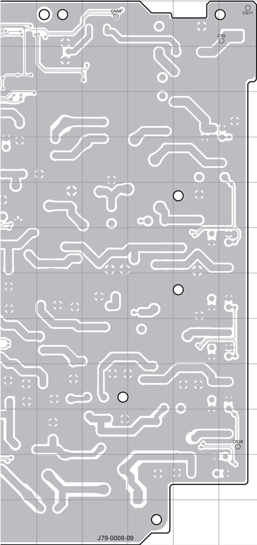
FINAL UNIT (X45-3780-20) Foil side view (J79-0008-09)
