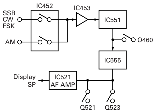
Fig. 6 From detection circuit to speaker output
